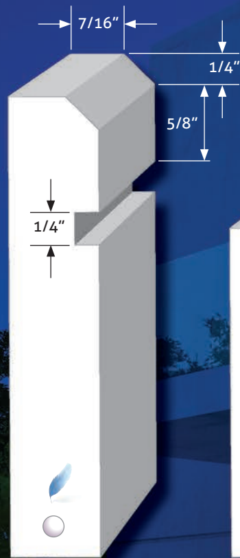
MCC312 11/16" x 3-1/2"
